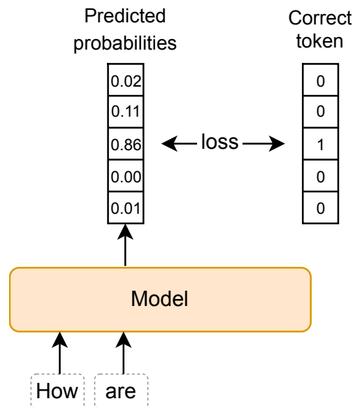
Figure 26: Loss calculation
