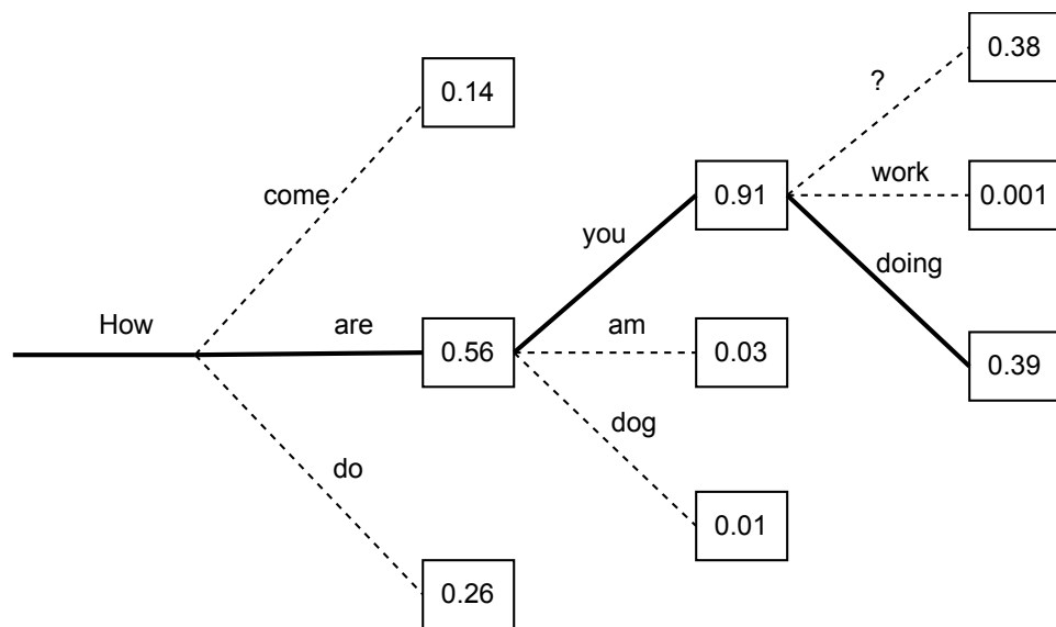
Figure 33: Greedy search
